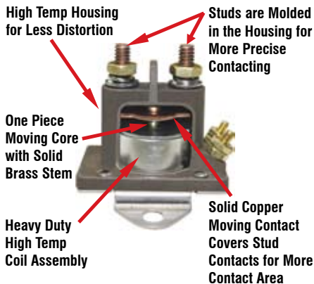
ARC SW058HD COIL & CONTACT ASSEMBLY
